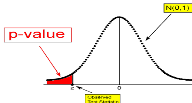
Fig.4: P-value for One-tailed Z-Test
