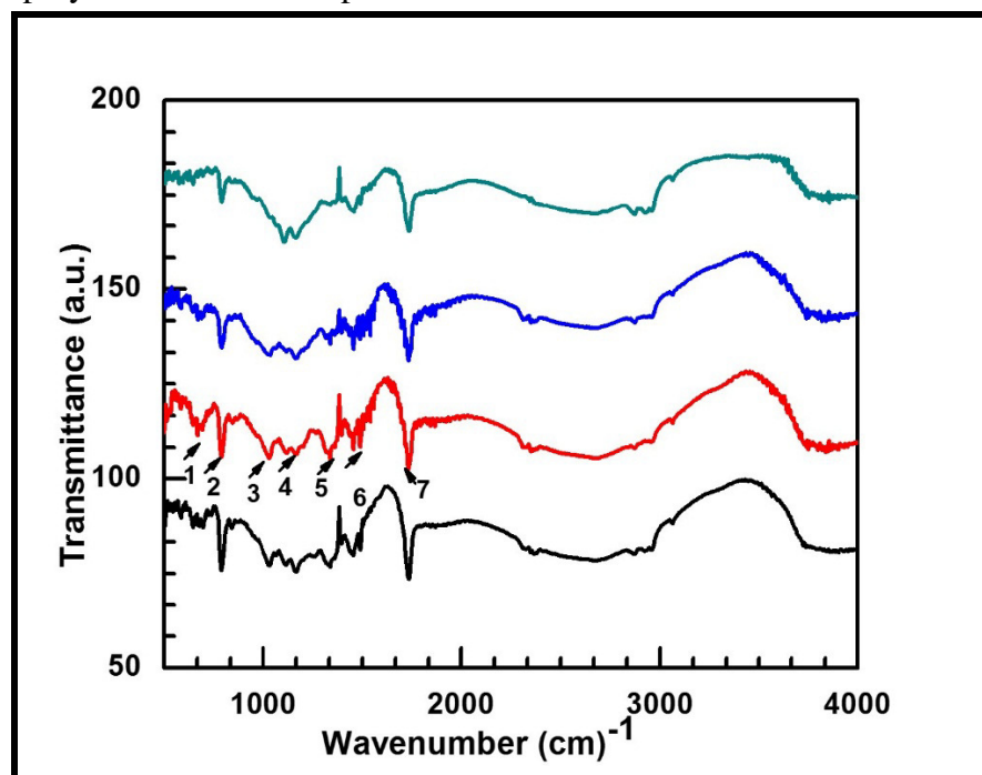
Fig. 1. FTIR spectra of polythiophene thin films deposited at (a) 0.5, (b) 1.0, (c) 1.5 and (d) 2.0 M thiophene concentration.
