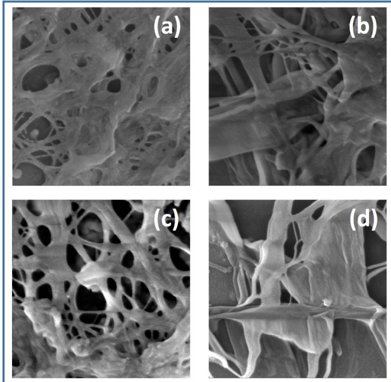
Fig. 2 FESEM micrographs of polythiophene thin films deposited at (a) 0.5, (b) 1.0, (c) 1.5 and (d) 2.0 M thiophene concentration.
