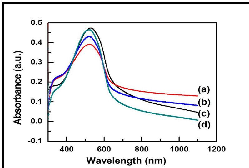
Fig. 3. UV-Visible spectra of polythiophene thin films deposited at (a) 0.5, (b) 1.0, (c) 1.5 and (d) 2.0 M thiophene concentration.
